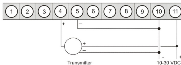
M2 in combination with a 3-wire-sensor 0/4-20 mA
