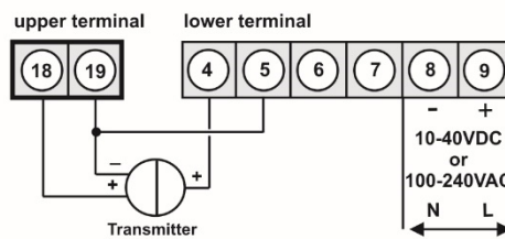
3-wire sensor 0-20 mA
