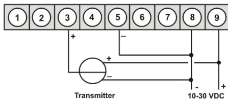
M3 in combination with a 3-wire sensor 0-10 V
