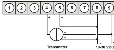
M3 in combination with a 3-wire sensor 0/4-20 mA
